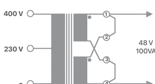
PARALLEL CONNECTION
