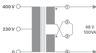
SERIAL CONNECTION
